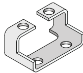
MOUNTING BRACKET 0.52" 32751
